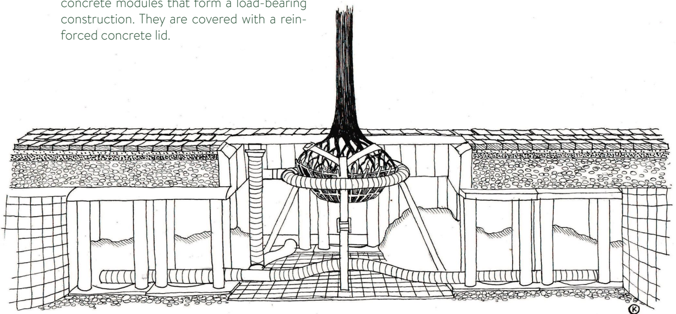
Figure 21: Example of installed soil cells system around a newly planted tree.
